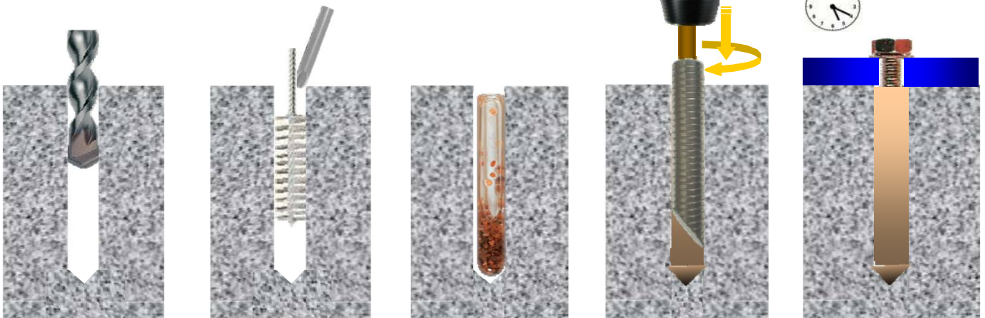
Drill correct diameter hole to correct depth
