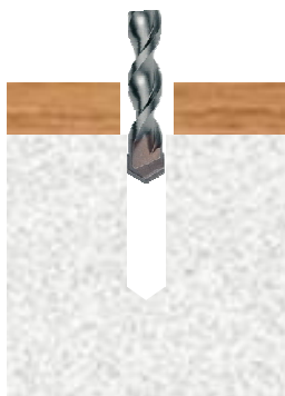
Position fixture and drill correct diameter hole to correct depth
